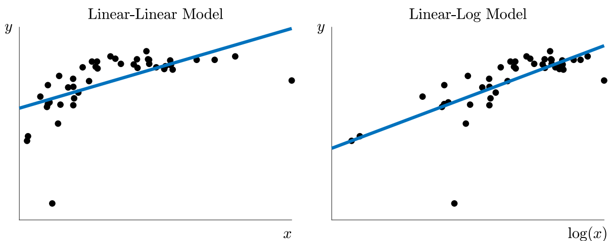
FIGURE 1: Using \log(x) as the horizontal axis gives a more linear shape to the data, thereby making it more appropriate for a linear regression.
